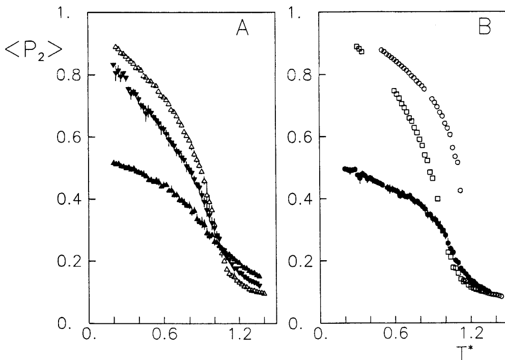
FIGURE 2 The second rank order parameter \langle P_2 \rangle_\lambda vs reduced temperature of a TBC droplet with N = 304 particles and strength parameter J , J = 1 (▲), J = 0.5 (▼), J = 0.25 (△) (plate A). We also show on plate B a CMC (○) and an empty space boundary, J = 0 , (□) simulation and a N = 1568 , J = 1 (●) against reduced temperature T^* = kT/\epsilon .
